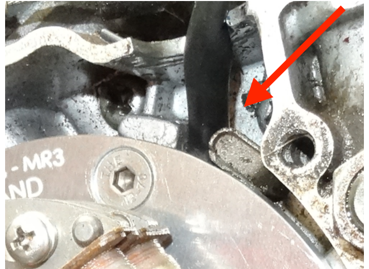
4. Ensure the wire is behind the retaining clip. Refit the fly-wheel and ensure the wire is not rubbing on the flywheel. Torque tighten to the Yamaha specification.
