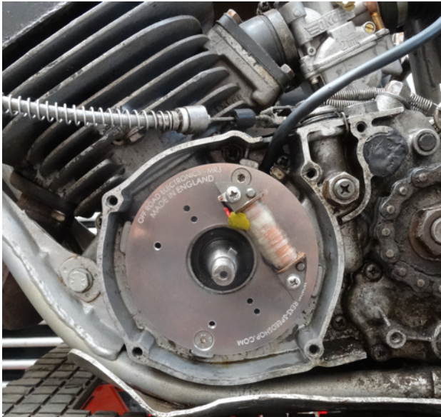
3. Fit the electronic ignition stator with windings in the 2 O'clock position as shown.
